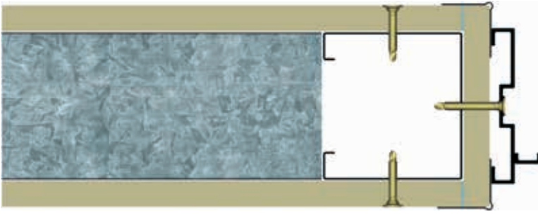
■ TYPICAL DETAIL FOR ALUMINIUM DOOR FRAME SECURED TO DUPLEX STUD®. DETAIL IS SIMILAR FOR ALUMINIUM GLAZING
