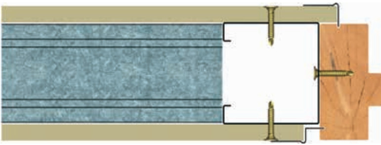
■ TYPICAL DETAIL FOR TIMBER DOOR FRAME SECURED TO DUPLEX STUD® WITH OPTIONAL SHADOWLINE DETAIL SHOWN
