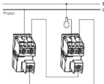
3/2-way switch
