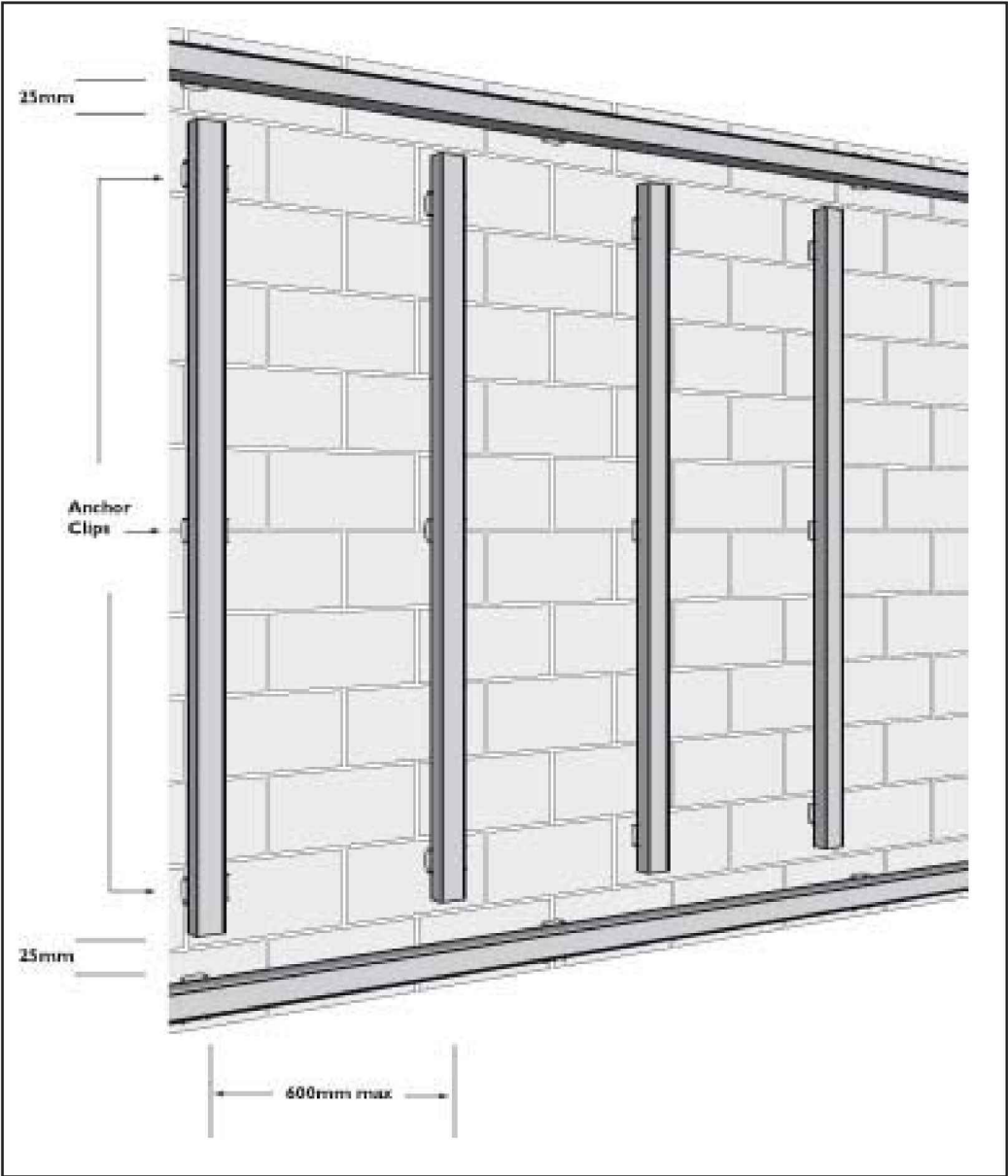
FIGURE 19: MASONRY WALL BATTENS
