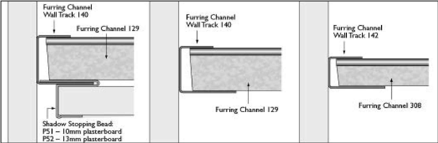
FIGURE 9: Furring Channel Wall Tracks
