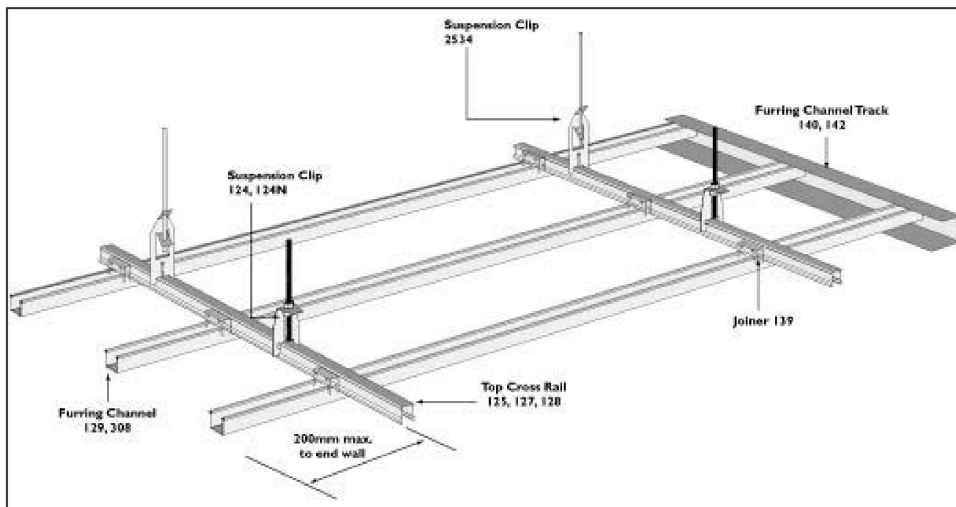
FIGURE 7: KEY-LOCK® Suspended Ceiling
