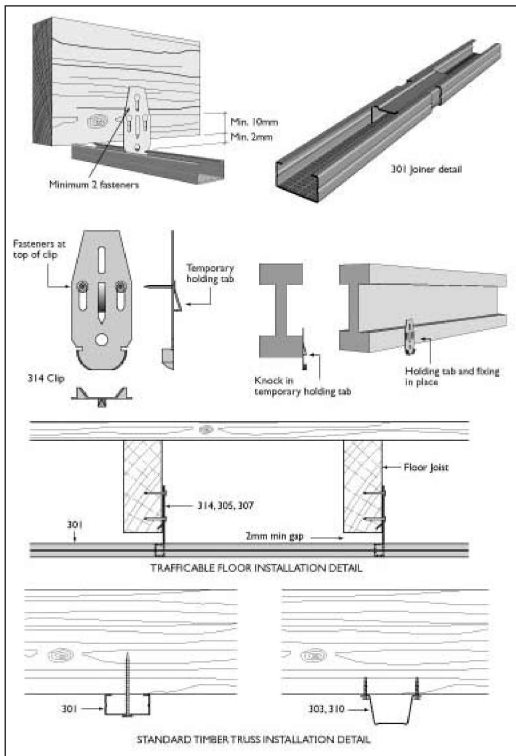
FIGURE 17: Metal Ceiling Battens
