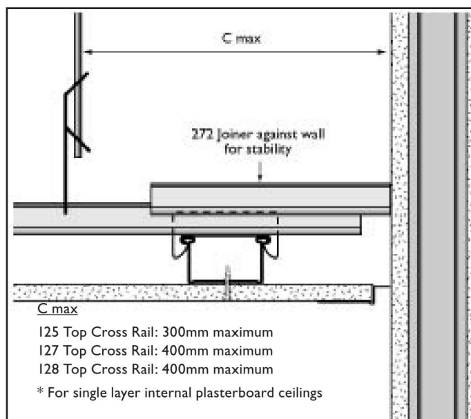
FIGURE 4: Stabilising the system
