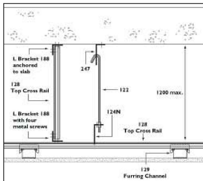
FIGURE 11: Downstrut Detail
