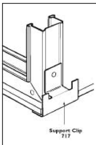
FIGURE 13: Support Clips
