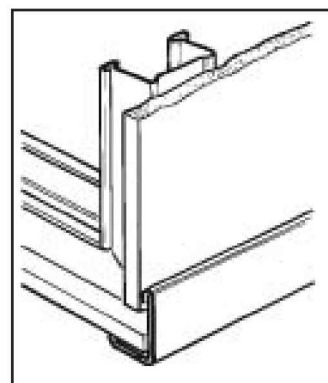
FIGURE 16: Vertical Members
