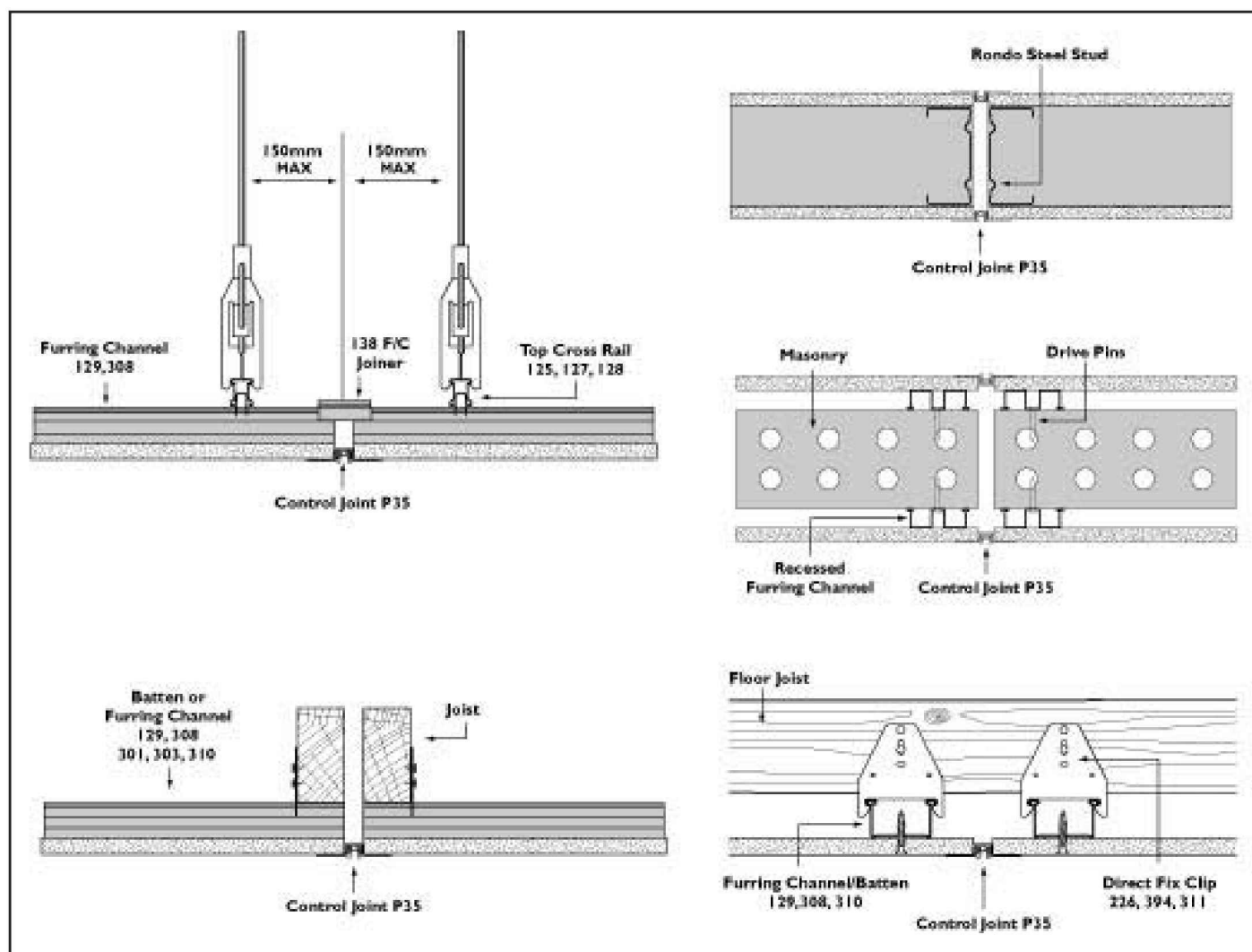
FIGURE 10: Control Joints
