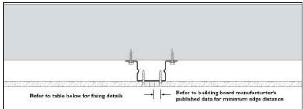
FIGURE 22: FIXING DETAIL
